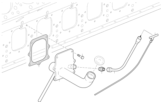
OIL FILLER NECK UPC.06G04 1402
