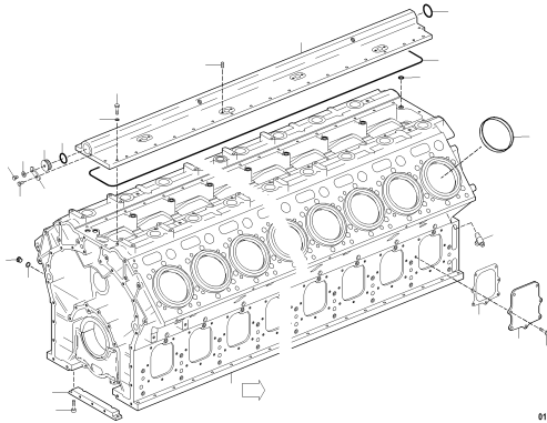
CRANKCASE UPC.06A01 2081
